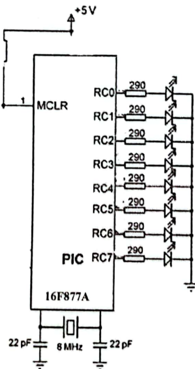
Figure 02: PIC diagram
